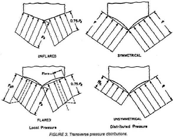
Figure 3. Transverse pressure distributions.
