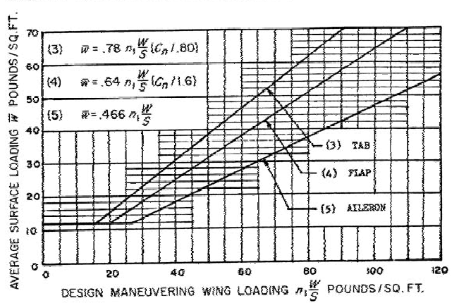
FIGURE 6 - AVERAGE LIMIT CONTROL SURFACE LOADING
