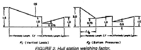
FIGURE 2. Hull station weighing factor.
