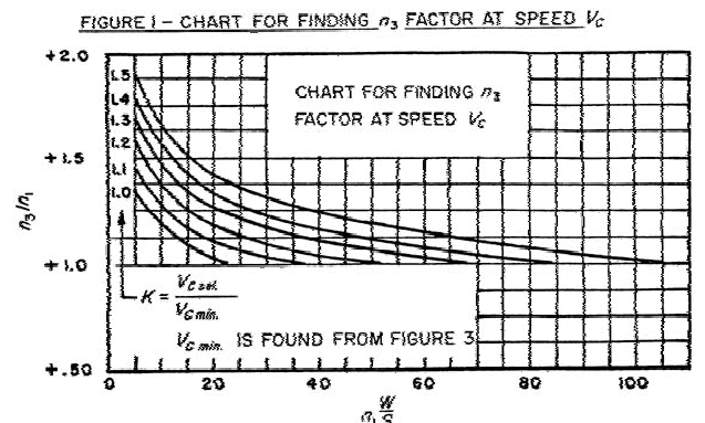
Figure A1 - Chart for finding n_3 factor at speed V_C .
