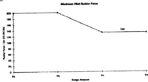
Figure 1. Maximum Pilot Rudder Force.
