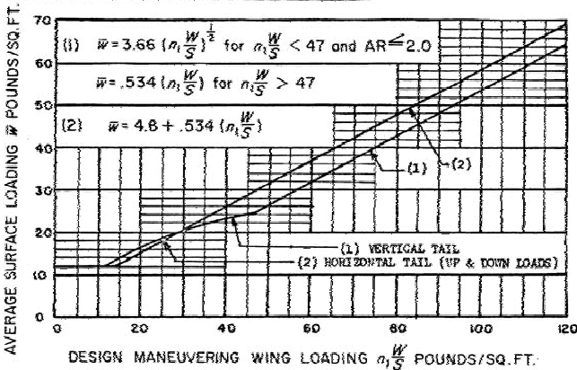
FIGURE 5 - AVERAGE LIMIT CONTROL SURFACE LOADING
