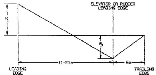
Figure A7—Chordwise Load Distribution for Stabilizer and Elevator or Fin and Rudder
