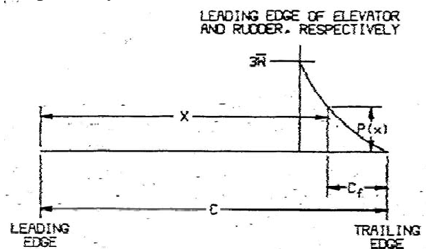
Leading Edge of Elevator and Rudder, Respectively
