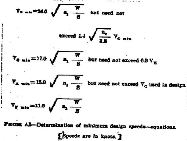
Figure A3 - Determination of minimum design speeds - equations. Speeds are in knots.
