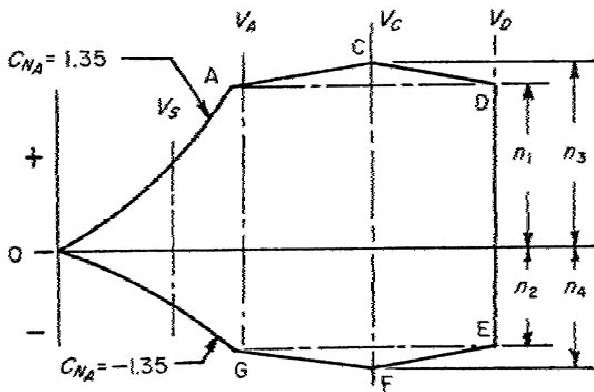
FIGURE 4—FLIGHT ENVELOPE
