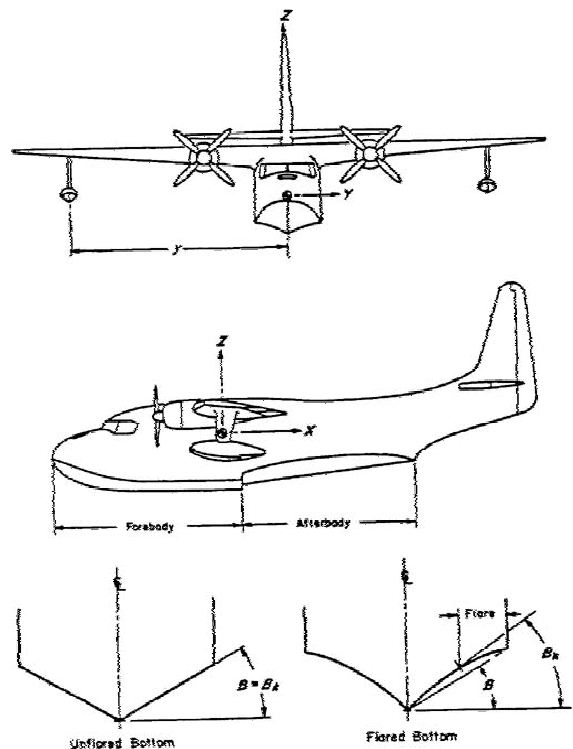
FIGURE 1. Pictorial definition of angles, dimensions, and directions on a seaplane.
